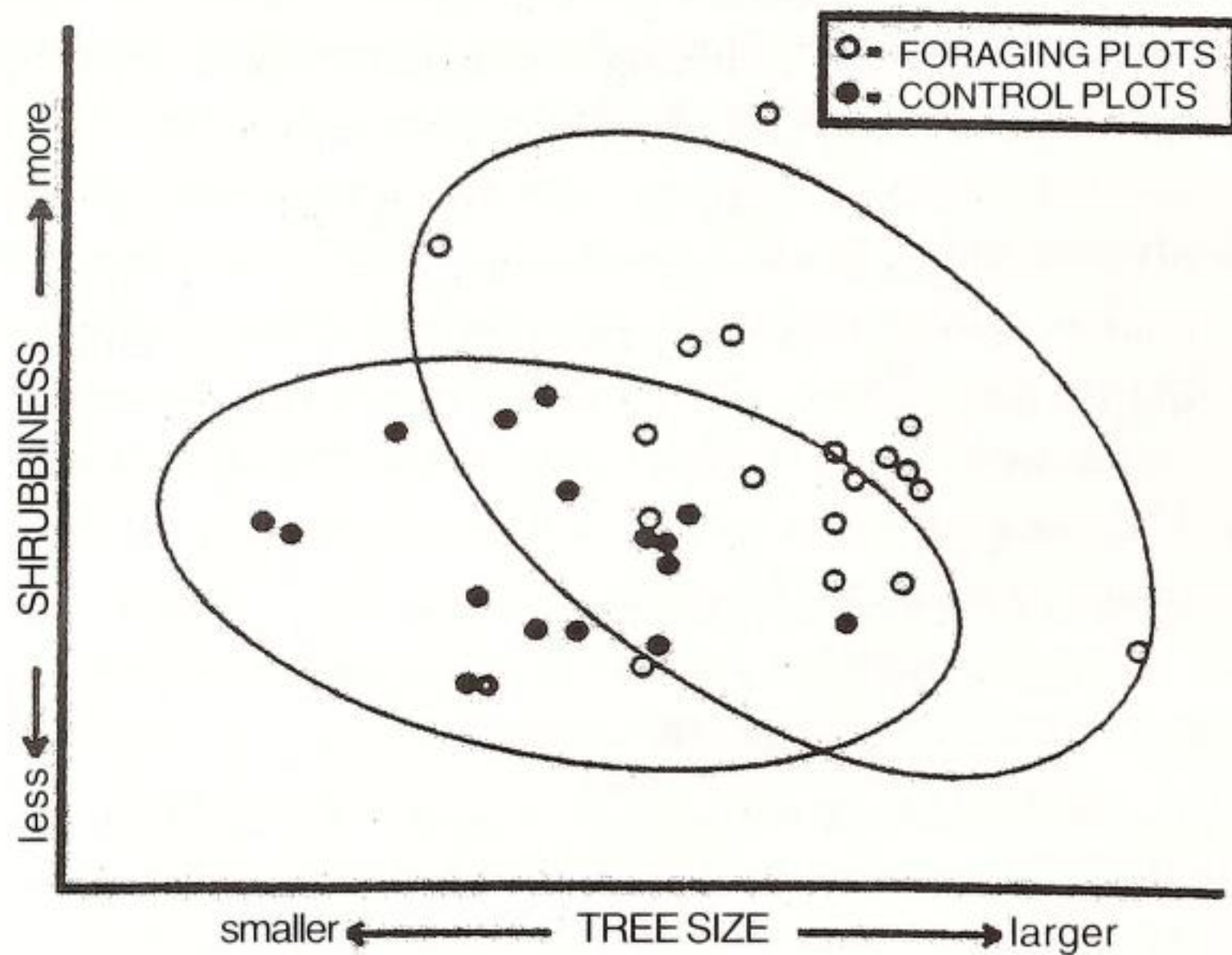
Fig. 1: Ordination, with 95% confidence ellipses, of fig tree foraging plots used by the Great Pied Hornbill and control fig tree plots, based on the scores of the first (tree size) and second (shrubiness) Principal Components.
